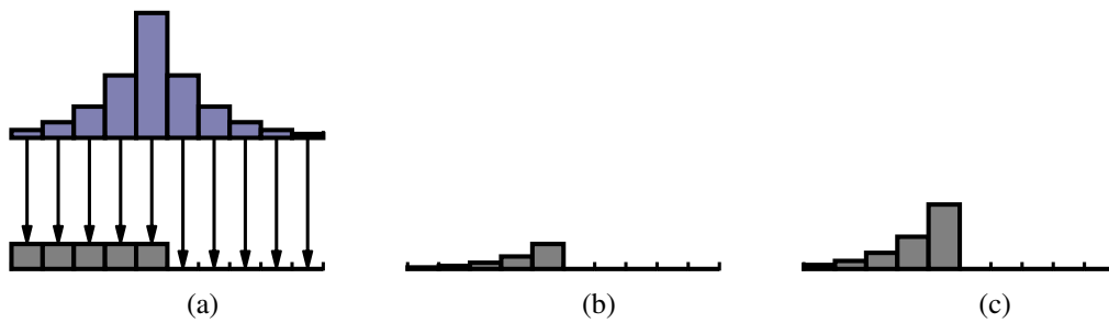
Figure 5.6: Using Bayes' rule to update state estimates based on a sensor reading. (a) The bar graph on the top represents the sensor model P(Z = True | X) . The bar chart on the bottom represents the prior distribution over the robot's location P(x) . The vertical arrows represent multiplication: the value of the sensor model at each state is multiplied by the prior probability for the corresponding state. (b) The resulting products. Note that these values do not sum to one. (c) The values at each state re-scaled (or normalized ) to make the total sum to 1. The result is the posterior probability distribution P(X | Z) .
