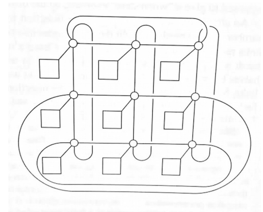
Toroidal Mesh
