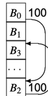
Slow Layout
