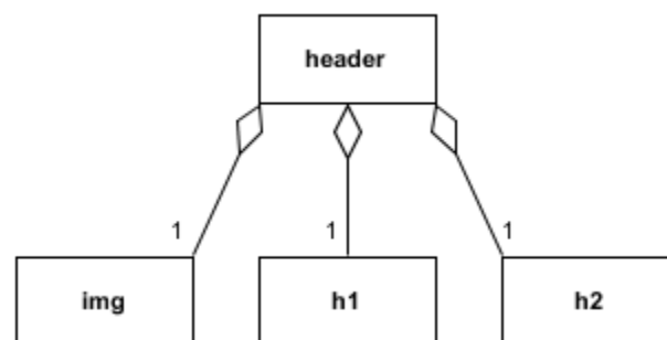
Figure 2 Structure of the header Element
