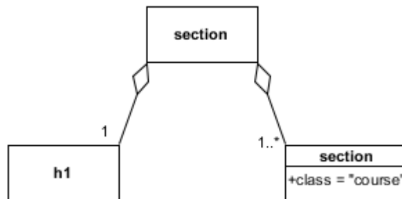
Figure 4 Structure of “Grouping” section Elements
