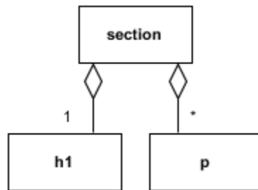
Figure 3. Structure of the section Element
