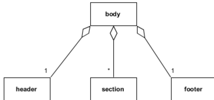
Figure 1 Structure of the body Element
