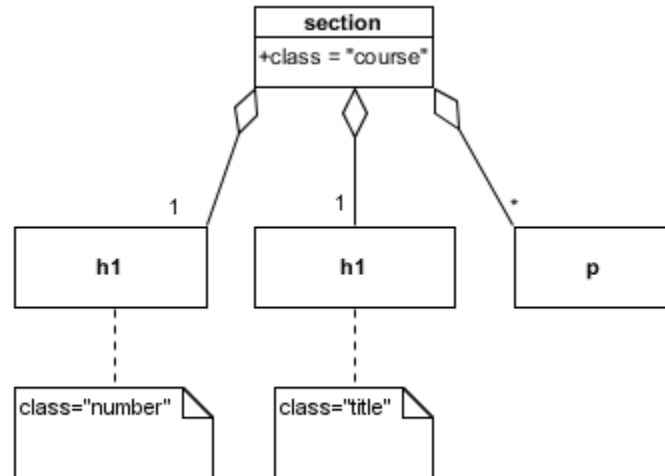
Figure 5. Structure of section Elements of Class course
